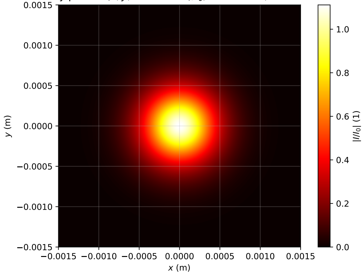
Intensity profile I(x, y, z = 0.796m)/I_0 , P_{in}=0.6P_{cr} , artificial time
